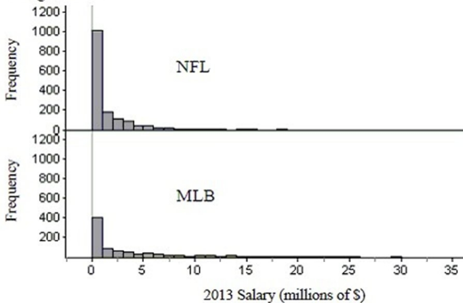
Histogram set 2
