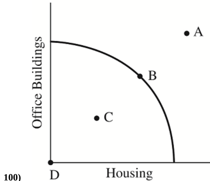
Figure – Production-Possibilities Curve
